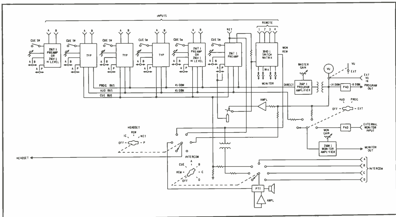
BLOCK DIAGRAM 212M-1
